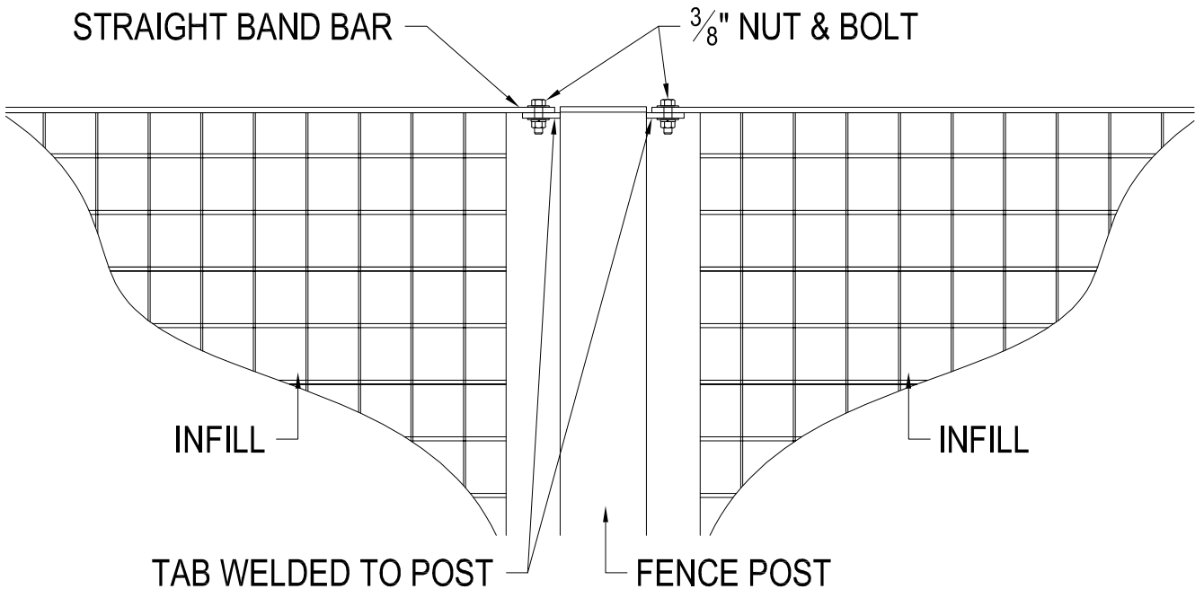
TYPICAL OPTIONS FOR CONNECTION OF ARCHITECTURAL PANELS
