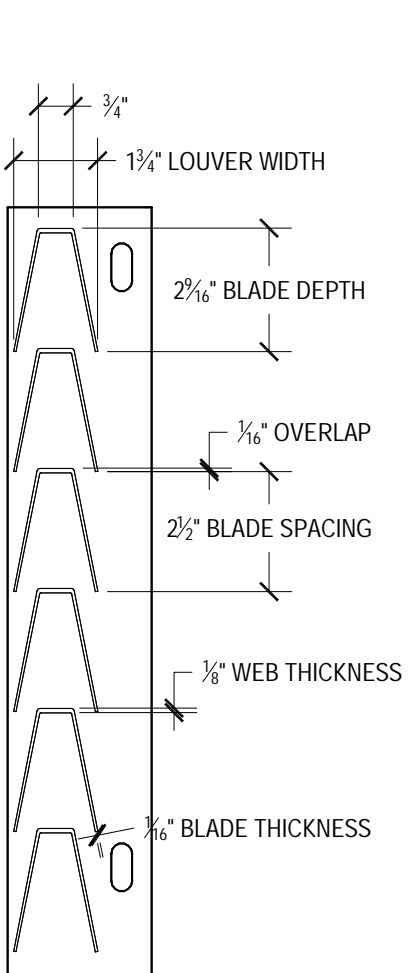
SECTION
